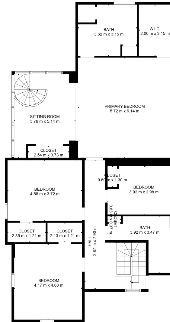
FLOOR 2
